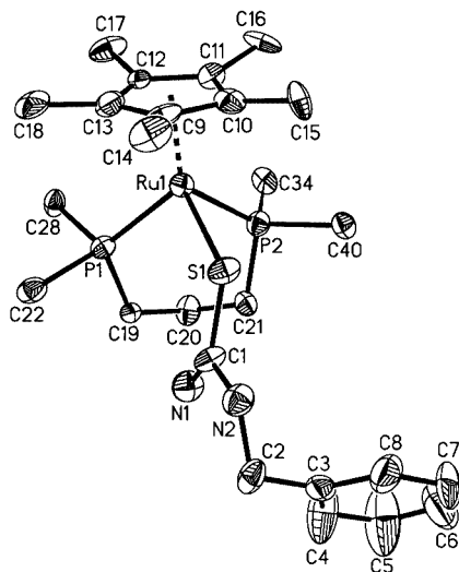
Figure 2. Structural drawing of 4 with thermal ellipsoids at the 30 % probability level; the four dppp phenyl groups and all of the hydrogen atoms have been omitted for clarity; selected bond lengths (Å): Ru(1)–S(1) 2.415(3), S(1)–C(1) 1.726(12), C(1)–N(1) 1.22(2), C(1)–N(2) 1.371(13); selected bond angles (deg): Ru(1)–S(1)–C(1) 126.0(4), S(1)–C(1)–N(1) 126.8(10), S(1)–C(1)–N(2) 112.4(9), N(1)–C(1)–N(2) 120.1(12).
