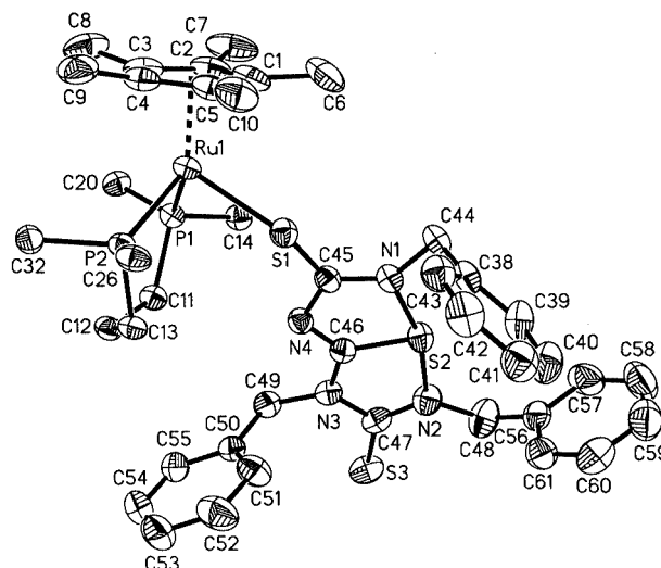
Figure 1. X-ray crystal structure of 3a with thermal ellipsoids at the 30 % probability level; the four dppp phenyl groups and all of the hydrogen atoms have been omitted for clarity; selected bond lengths (Å): Ru(1)–S(1) 2.4427(8), S(1)–C(45) 1.739(3), C(45)–N(1) 1.305(4), C(45)–N(4) 1.370(4), C(47)–N(2) 1.296(5), C(47)–N(3) 1.406(4), C(46)–N(3) 1.370(4), C(46)–N(4) 1.314(4), S(2)–N(1) 1.884(3), S(2)–N(2) 1.969(3), C(46)–S(2) 1.722(3), C(47)–S(3) 1.683(3); selected bond angles (deg): C(45)–S(1)–Ru(1) 126.56(10), N(1)–S(2)–C(46) 81.80(14), S(2)–C(46)–N(4) 120.4(2), N(3)–C(46)–S(2) 116.6(2), C(46)–N(4)–C(45) 110.9(3), C(45)–N(1)–S(2) 113.1(2), N(2)–C(47)–N(3) 109.8(3), C(46)–N(3)–C(47) 116.1(3), C(46)–S(2)–N(2) 82.79(14), S(2)–N(2)–C(47) 114.7(2), N(1)–C(45)–S(1) 122.4(2), N(4)–C(45)–S(1) 123.7(2), N(2)–C(47)–S(3) 128.2(3), N(3)–C(47)–S(3) 122.1(3).
